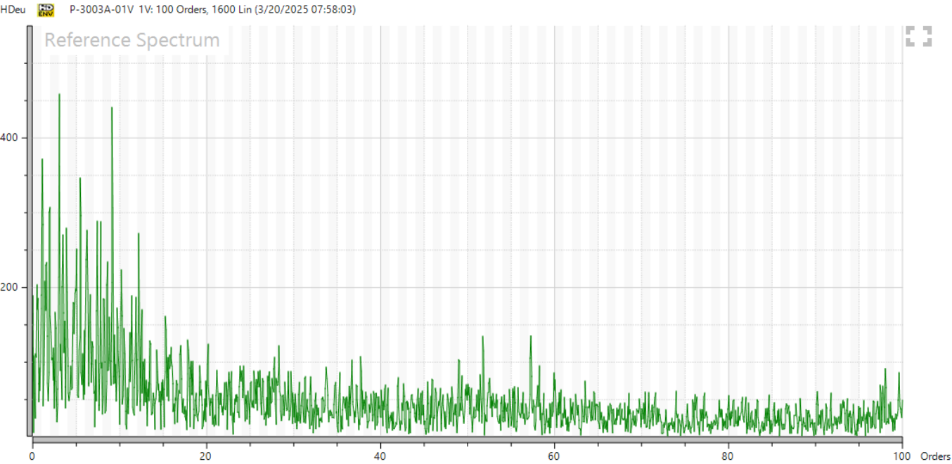
Before replacing the damaged bearing
